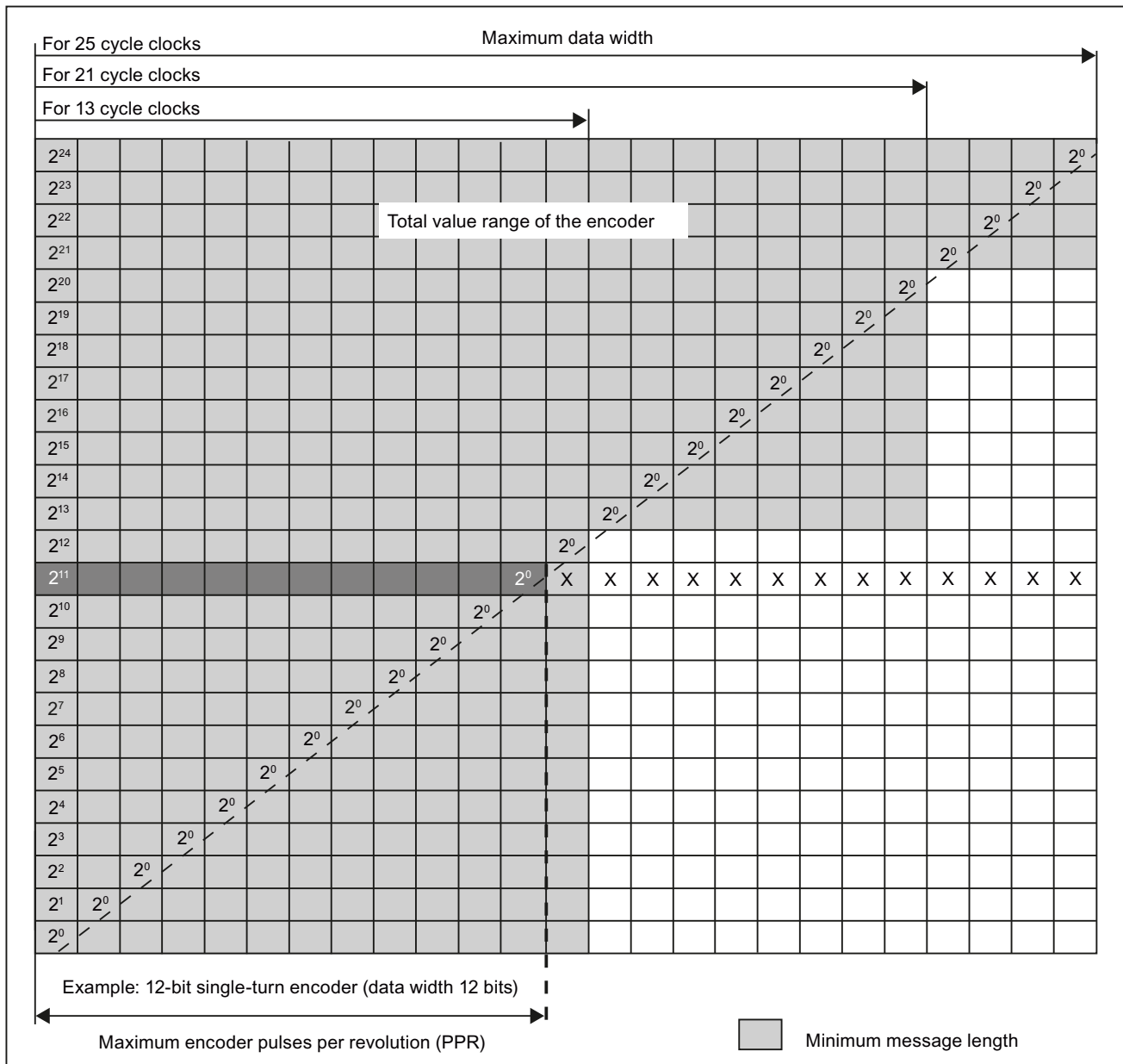
Figure 3-11 Right-justified profile
