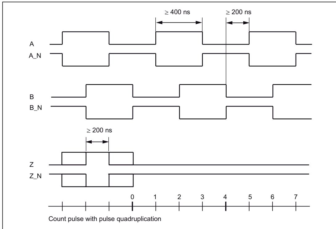
Figure 3-9 Signal forms of incremental encoders
