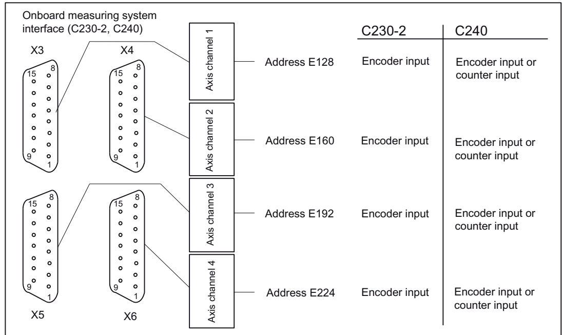
Figure 6-8 Addressing the onboard measuring system interface
