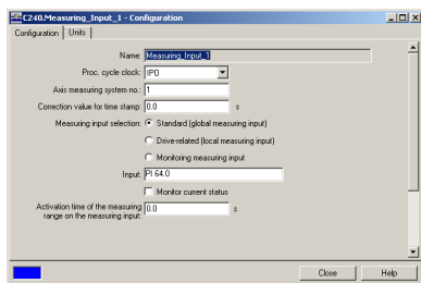
Figure 3-15 Configuration example for global measuring (without symbolic assignment)
