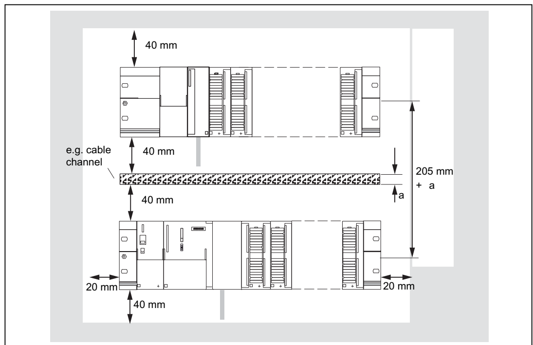
Figure 4-2 Clearances
