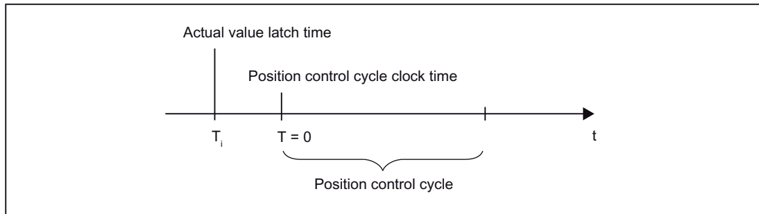
Figure 3-12 Position control cycle
