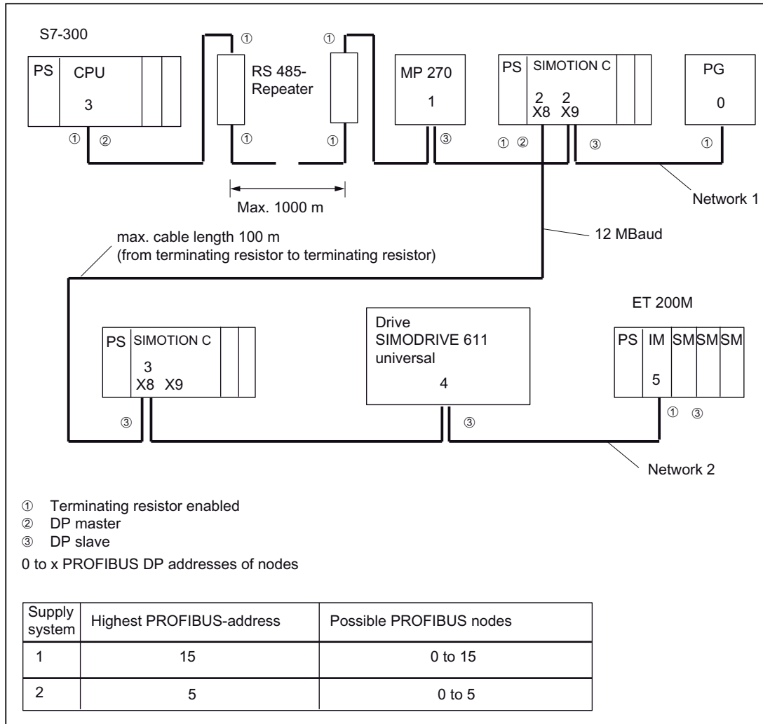
Figure 5-19 Networking example
