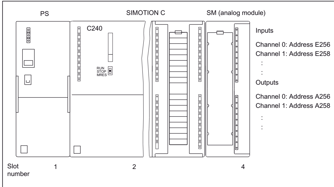
Figure 6-5 Addresses for the inputs and outputs of the analog module in slot 4
