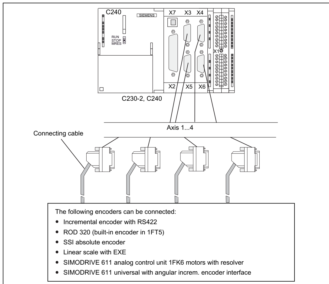
Figure 5-15 Encoder connections
