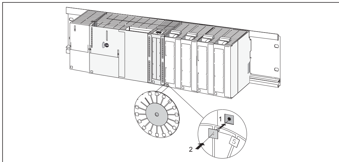
Figure 4-8 Inserting slot numbers on the modules
