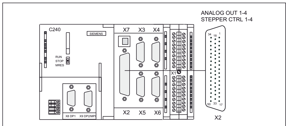
Figure 3-5 Position of the X2 connector
