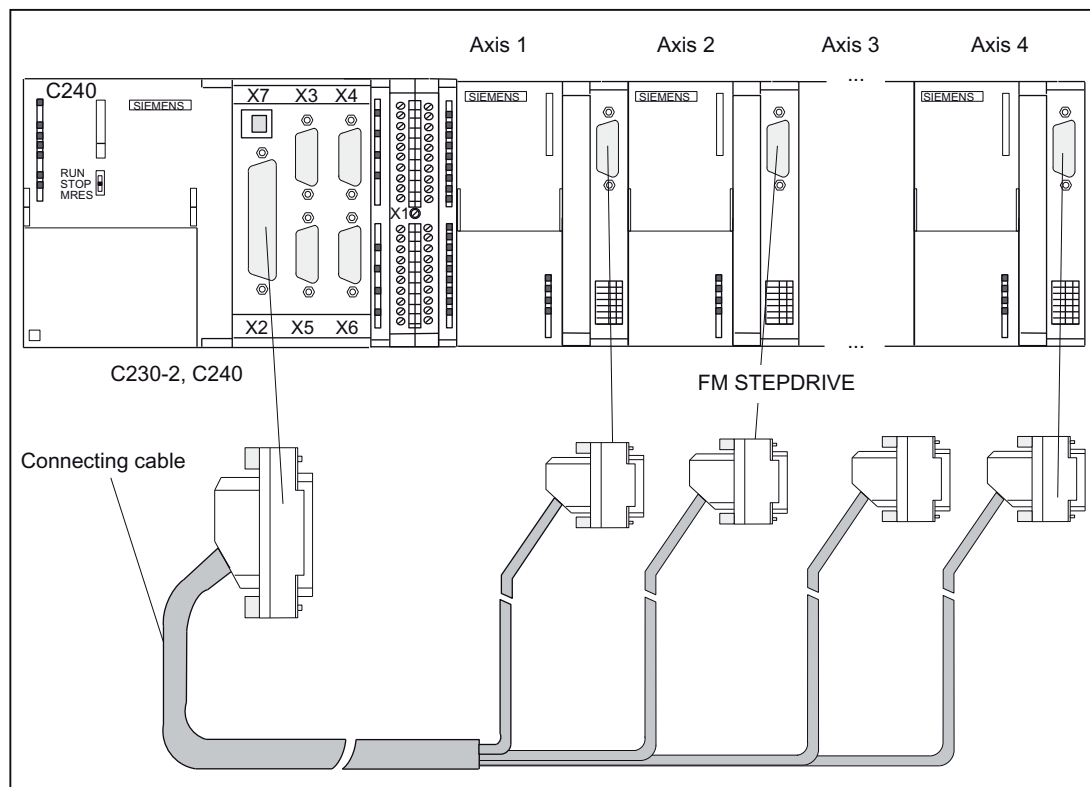
Figure 5-10 Connection of FM STEPDRIVE drive units
