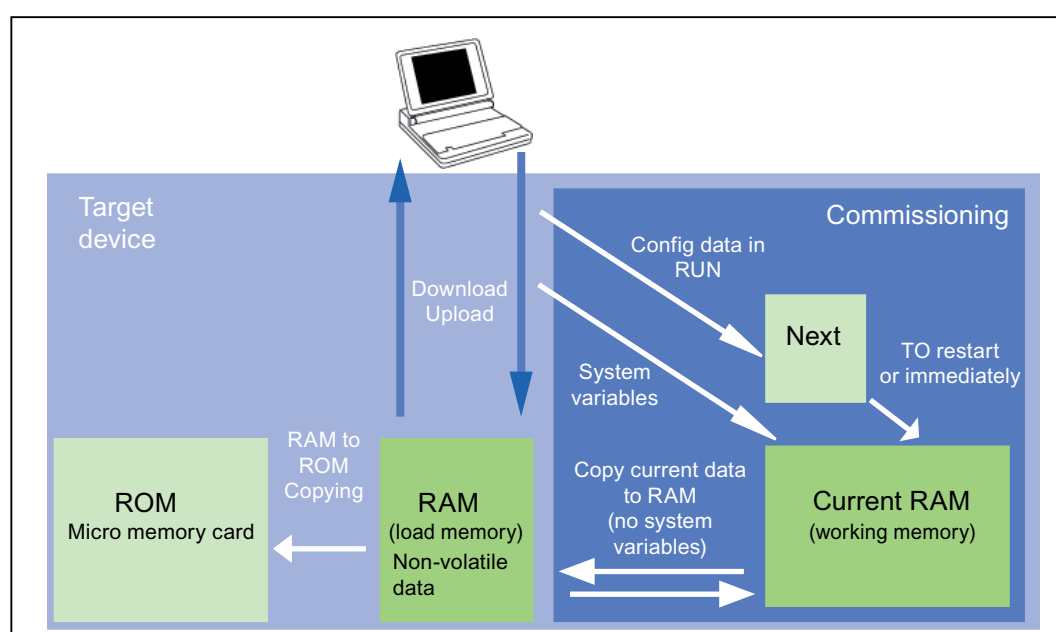
Figure 7-3 Configuration data and system variables on volatile memory
