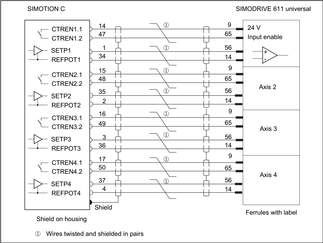
Figure 5-9 Terminal diagram for C230-2/C240 and SIMODRIVE 611 universal with analog setpoint interface
